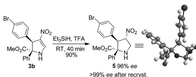
Scheme 2. Stereoselective reduction of the dihydropyrrole and X-ray crystallographic structure of 5 .TFA = trifluoroacetic acid.
